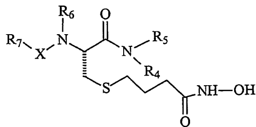
(IIIa)
